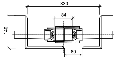
Expansion joint 40 mm
