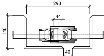
Expansion joint 80 mm
