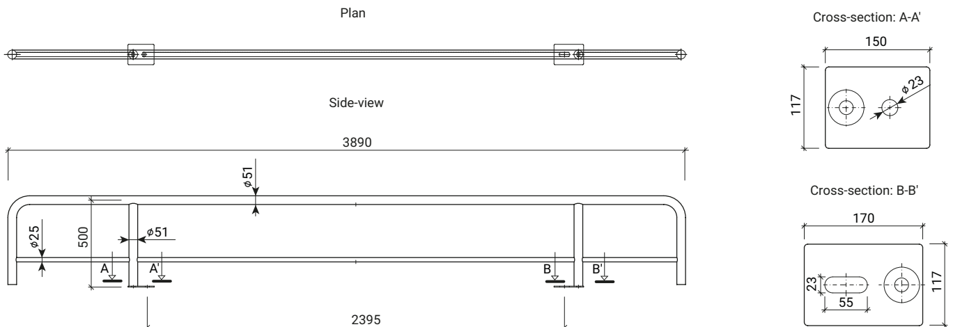
Nominal dimensions - basic shapes:
